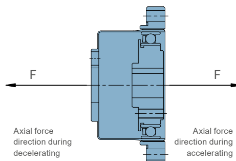
Axial force direction of the Wave generator
