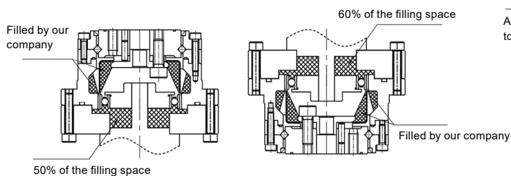
Regular FSS-U/C Grease Filling Amount (g)
