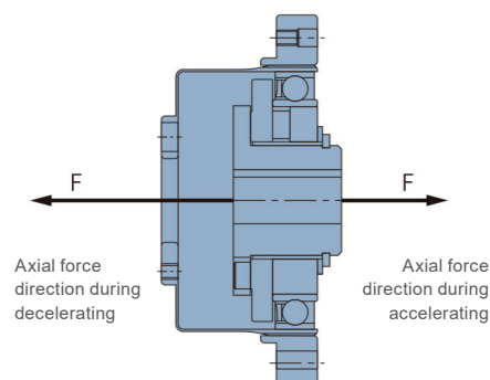
Axial force direction of the Wave generator
