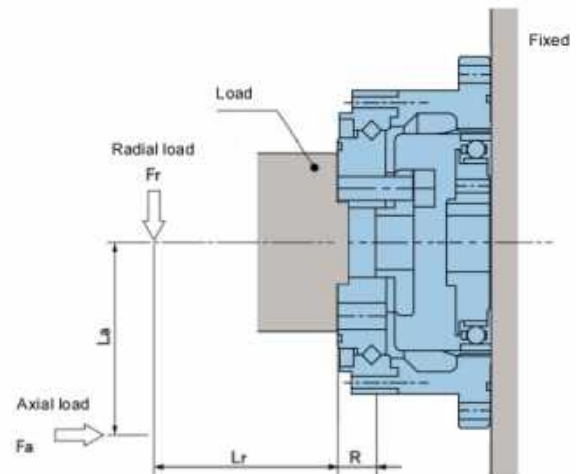
External Load influence diagram
